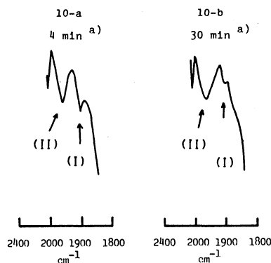
Fig. 10. IR spectra of the catalyst system of Fig. 6 obtained at the N/Rh ratio of 1. a) A time period from withdrawal of the reaction mixture from the autoclave to measurement for IR spectrum.
